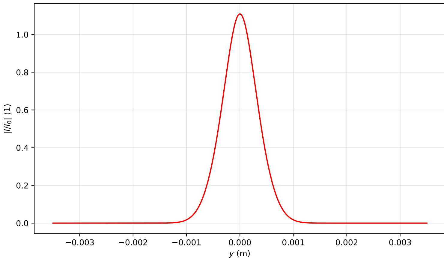
Intensity profile I(x=0, y, z=0.239)/I_0 , P_{in}=2.0P_{cr} , artificial time
